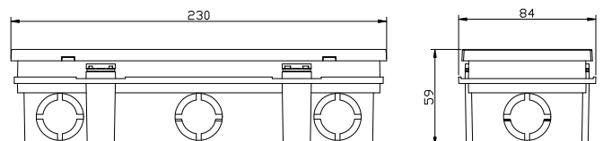
Recessed Model BLR6CT2
