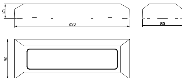
Surface Model BLR6CT2
