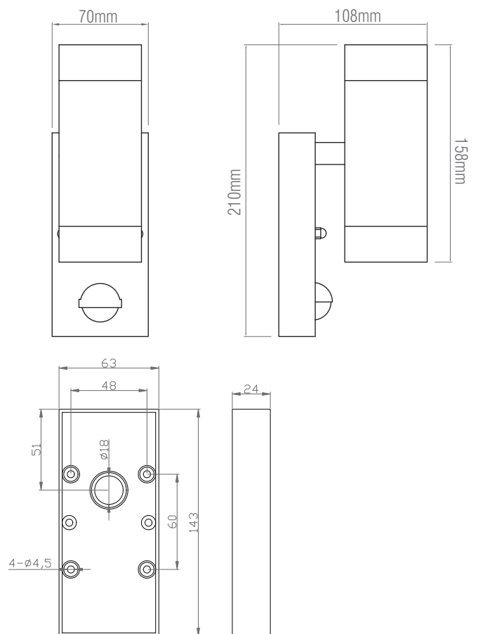
Wall back plate (Unit: mm)
